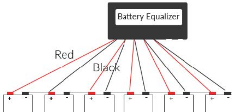
Figure 1: 6×12V battery bank
