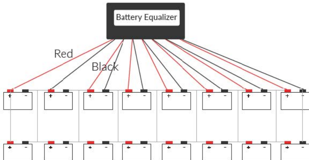
Figure 2: Multiples sets of batteries
