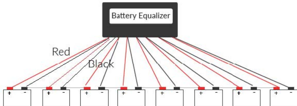
Figure 1: 8×12V battery bank
