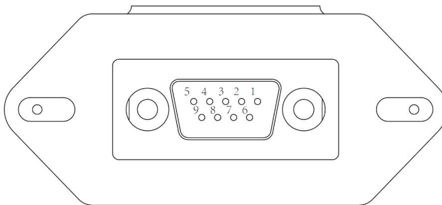
WIFI/RS232
